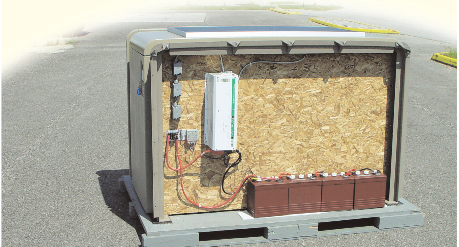
End panel covers Batteries and inverter
